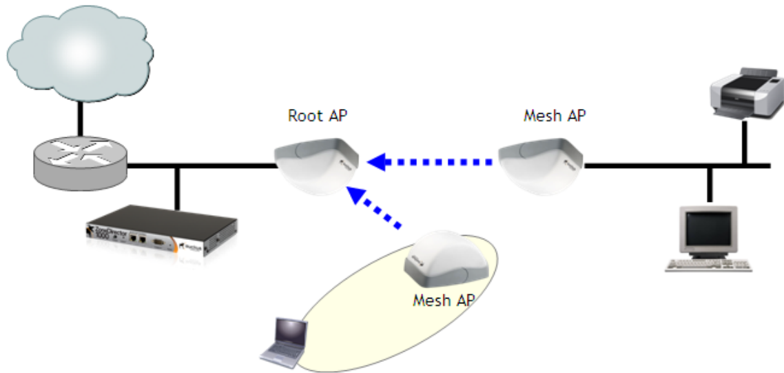
FIGURE 305 Mesh - wireless bridge topology
