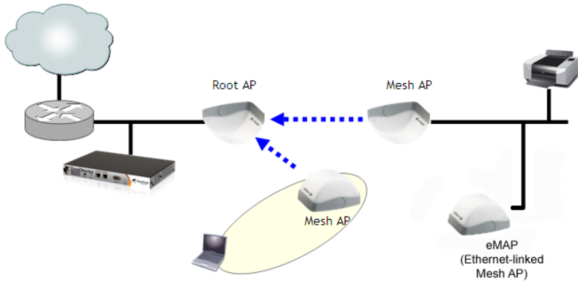
FIGURE 306 eMAP - Hybrid Mesh topology
