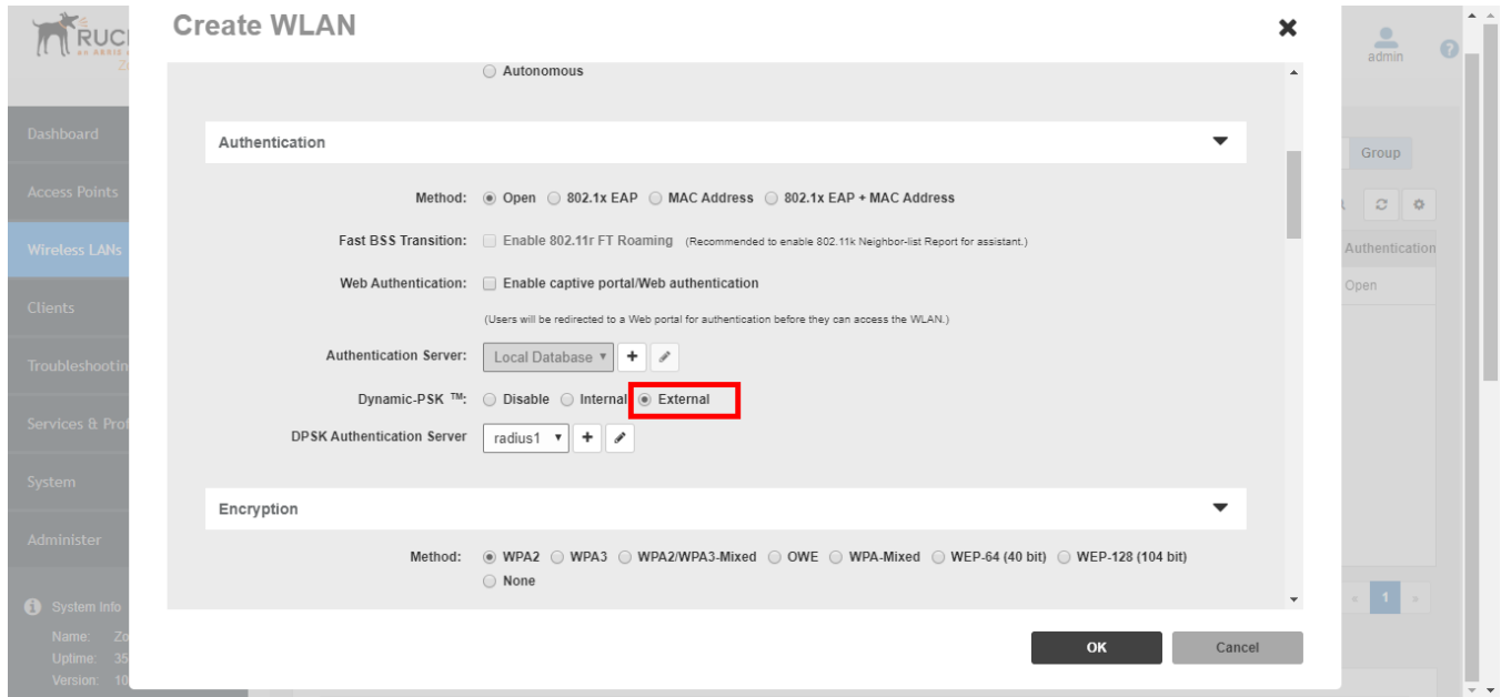
FIGURE 57 External DPSK
